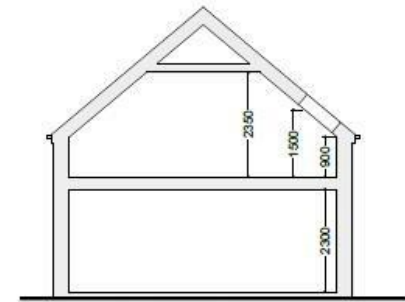
SECTION 1:100
